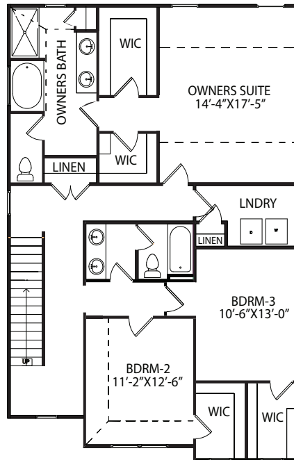
SECOND FLOOR NOT TO SCALE
